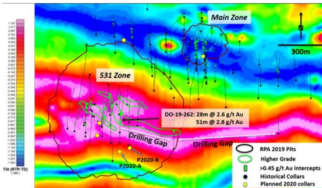
Fig. 2: Drill plan for greater 531 Zone area, on reduced to pole tilt derivative magnetics (RTP-TD) emphasizing lithological contacts. Note extensive drilling gap immediately to ESE and E of higher grade DO-19-262 intercepts; P2020-A is currently in progress.
