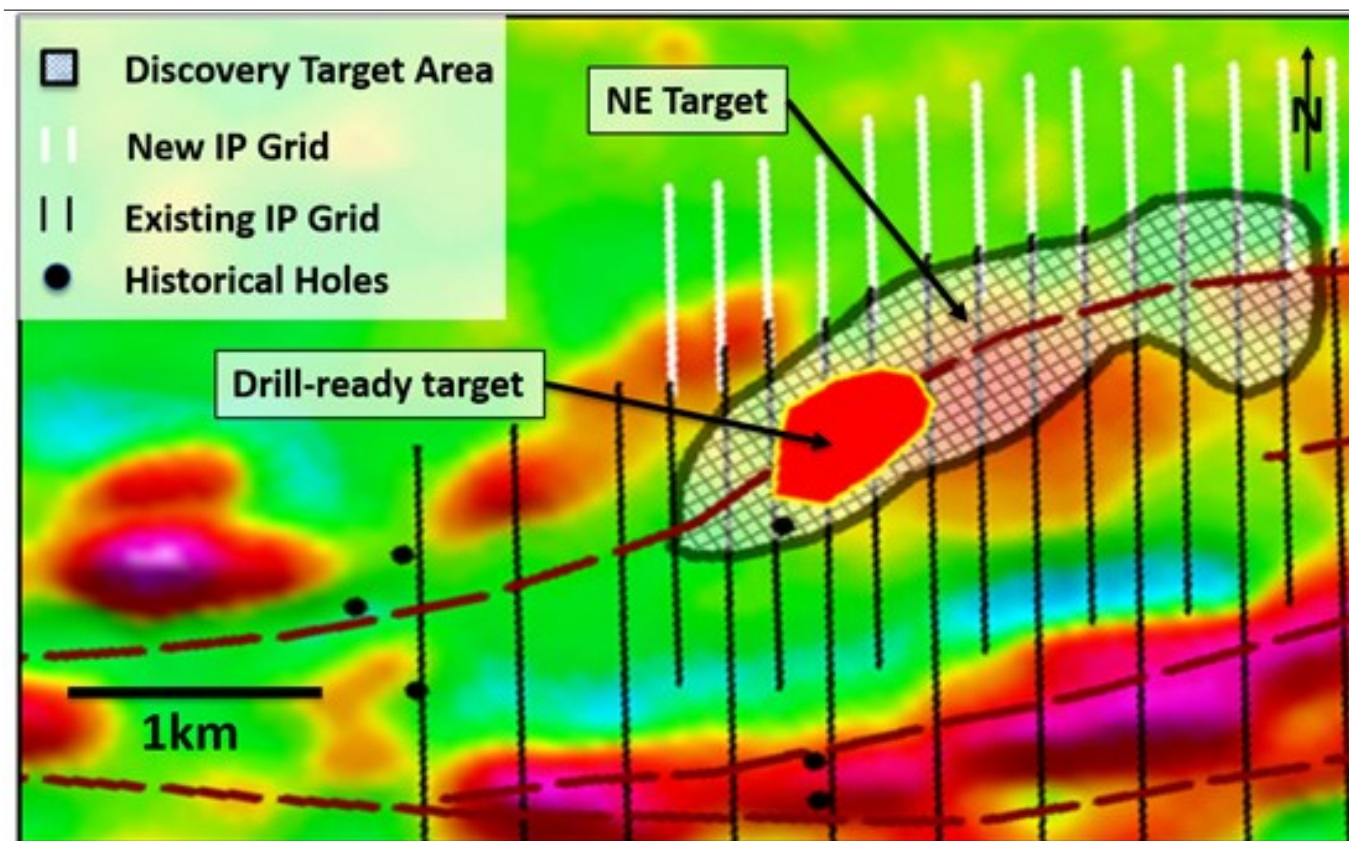
Fig. 2: NE target area trend of chargeability anomalies, on regional magnetic base and showing historical drillholes. Note only a single drillhole into the ~3km NE Target area.
